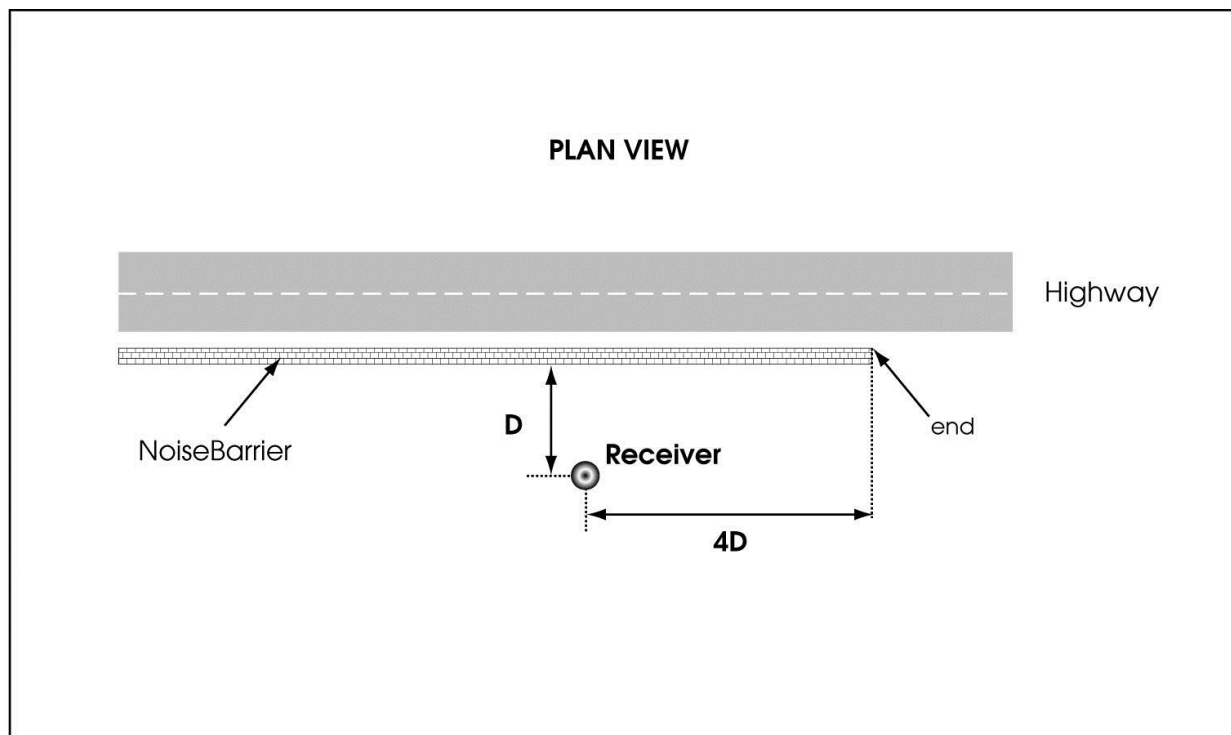
Figure 5-18. 4D Rule
