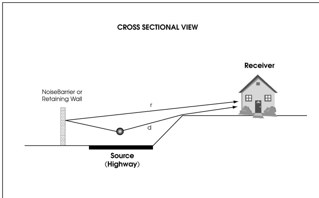
Figure 5-27. Single-Barrier Reflection (Direct Noise Shielded, Reflected Noise Not Shielded)
