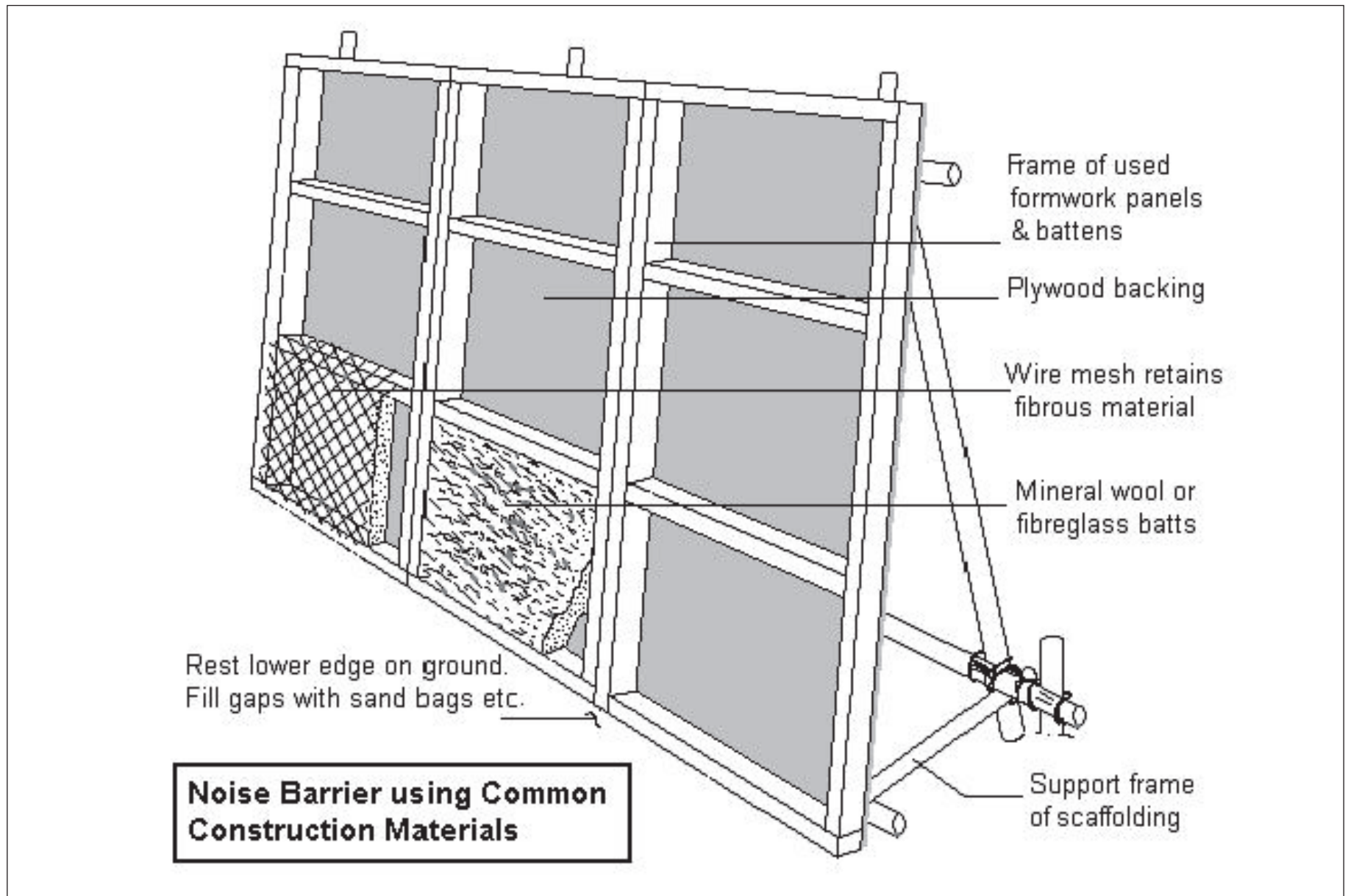
Figure 3.10-2 Temporary Noise Wall Barrier Construction
